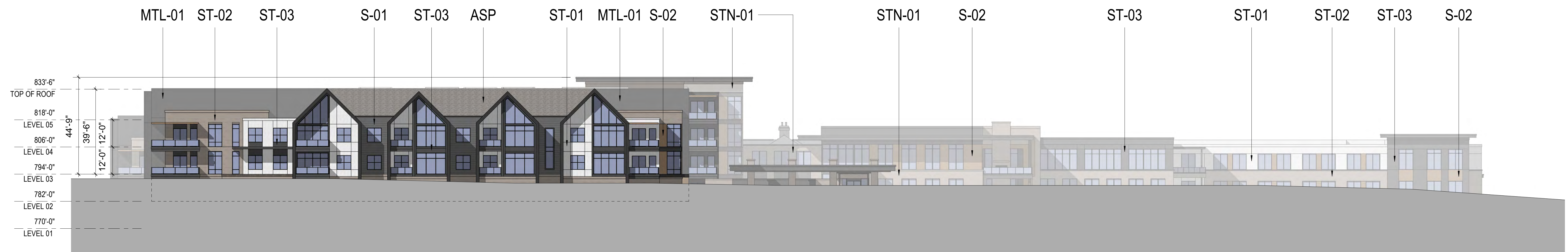
2 SOUTH ELEVATION (BOSTON STREET) 1" = 20'-0"
